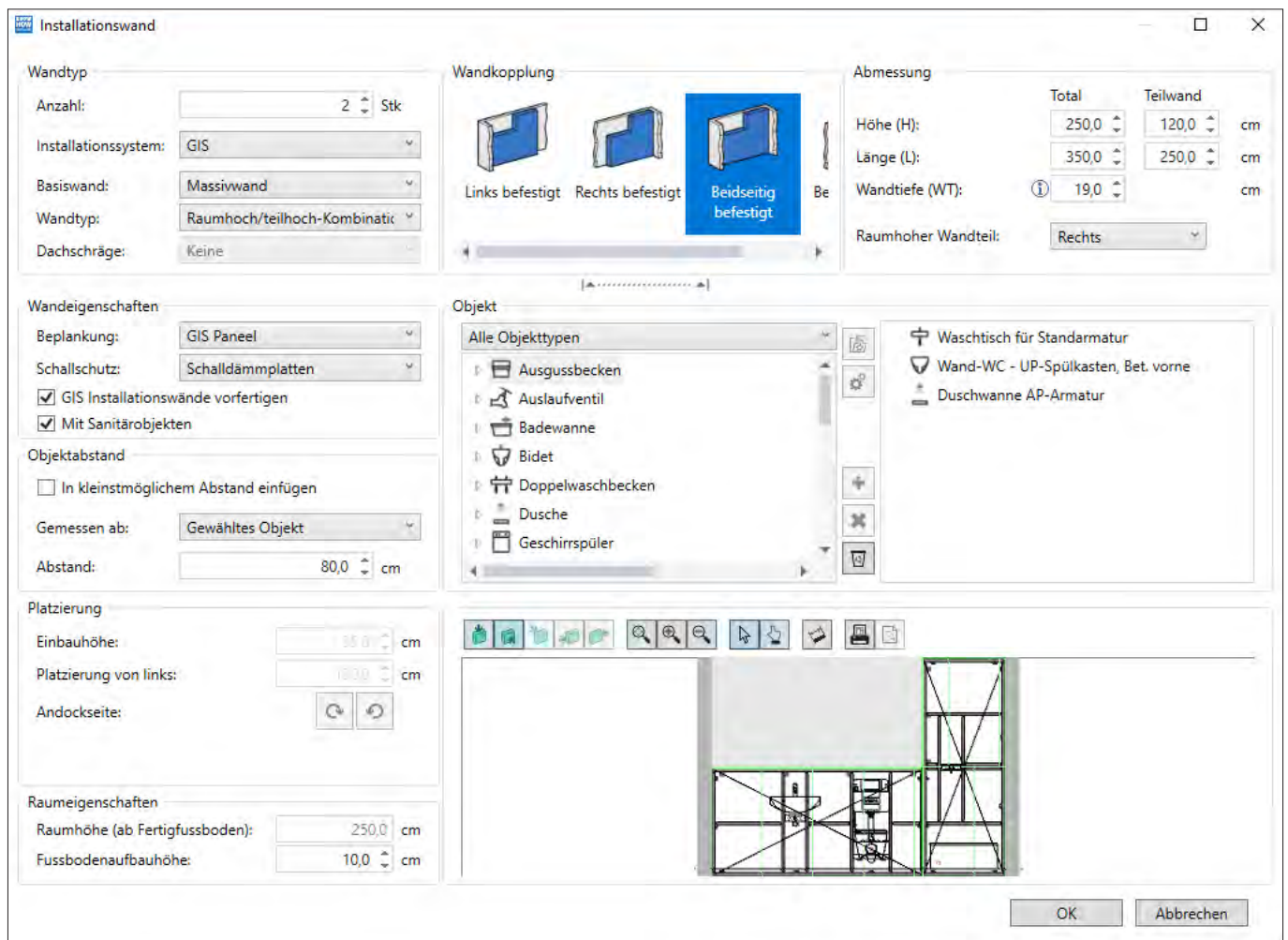
Figure 26: Planned Geberit GIS installation wall with washbasin, WC and shower (preview of 3D CAD export)
