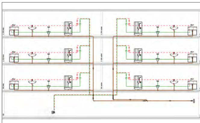
Figure 27: Planning a drinking water installation in the schematic drawing
