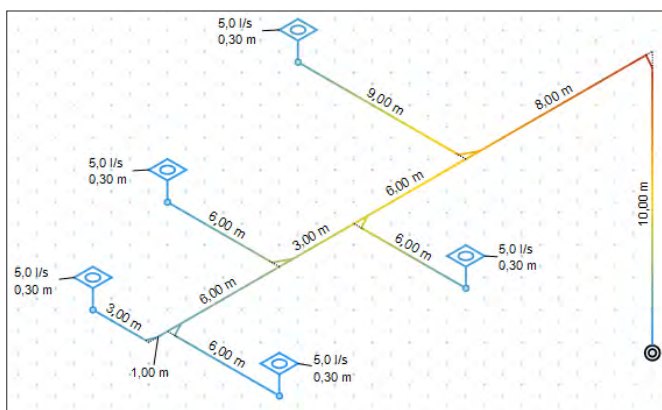
Figure 29: Roof drainage project with colour coding
